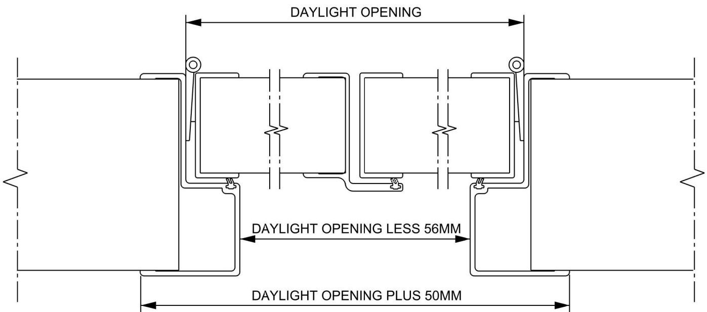
VIEW ON A-A
