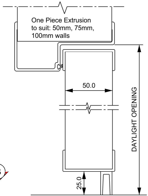
VIEW ON B-B
