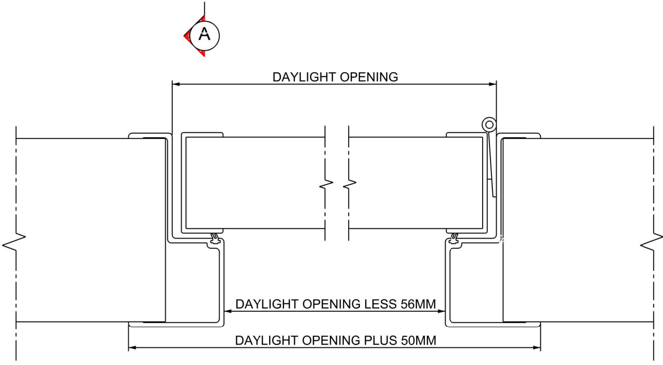
VIEW ON A-A
