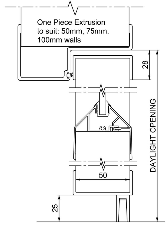
VIEW ON B-B
